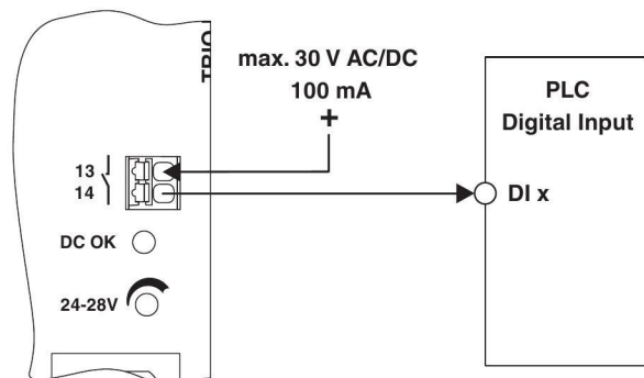
Figure 19 Wiring principle
