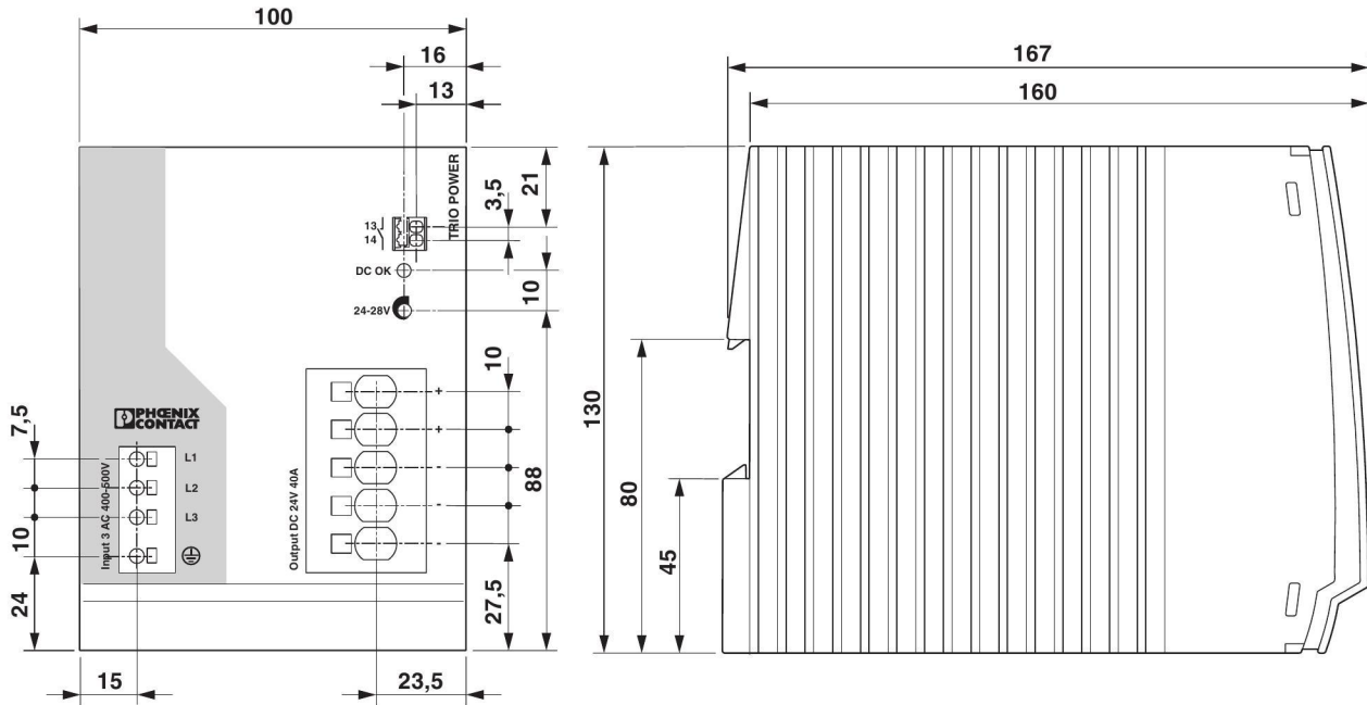
Figure 6 Device dimensions
